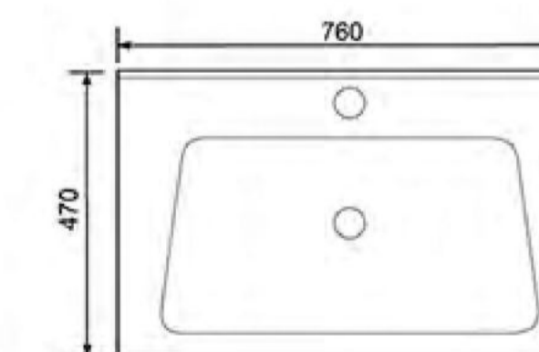
760 Counter Basin Size:760X470X200mm
